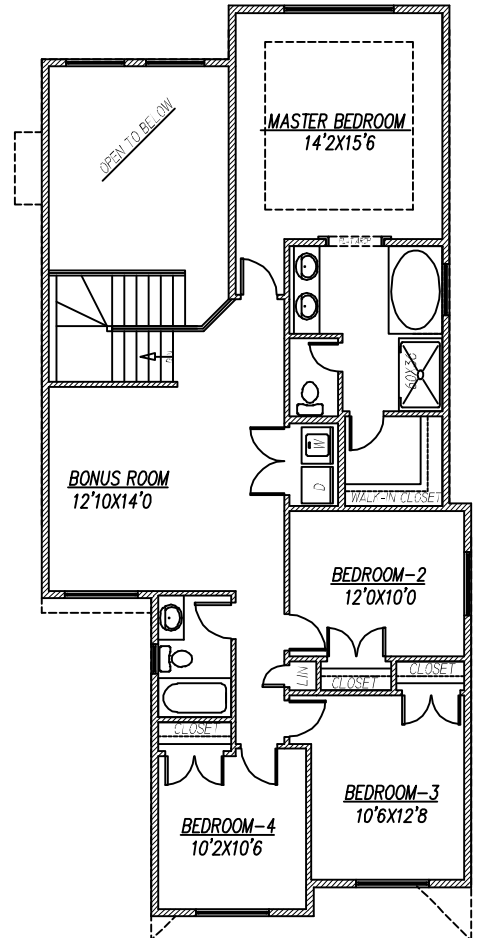
UPPER FLOOR PLAN 1292 SQ. FT.
