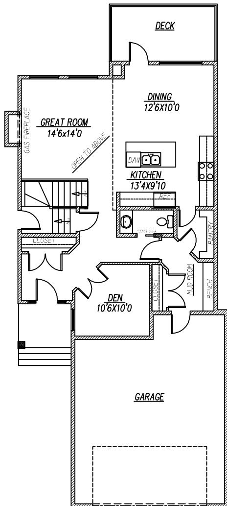
MAIN FLOOR PLAN 1007 SQ. FT.
